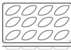
Boats art. 47742-50 mm. 72x30 h. 15 pcs 12
